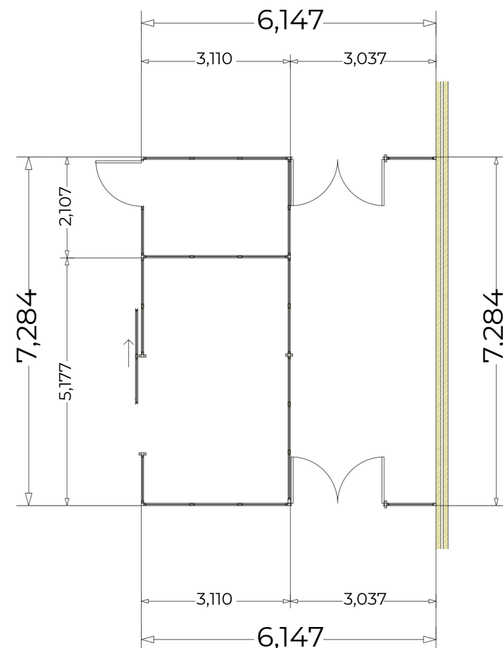
TYPICAL DOUBLES KIN FLOOR PLAN LAYOUT
