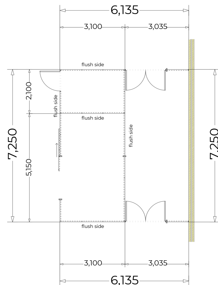
TYPICAL SINGLE SKIN FLOOR PLAN LAYOUT
